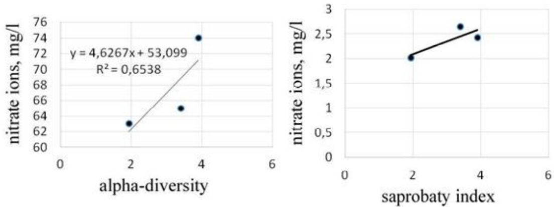
Figure 2. Dependence of biological indicators of macrophyte communities on nitrate ions ( \text{NO}_3^- ) concentration
