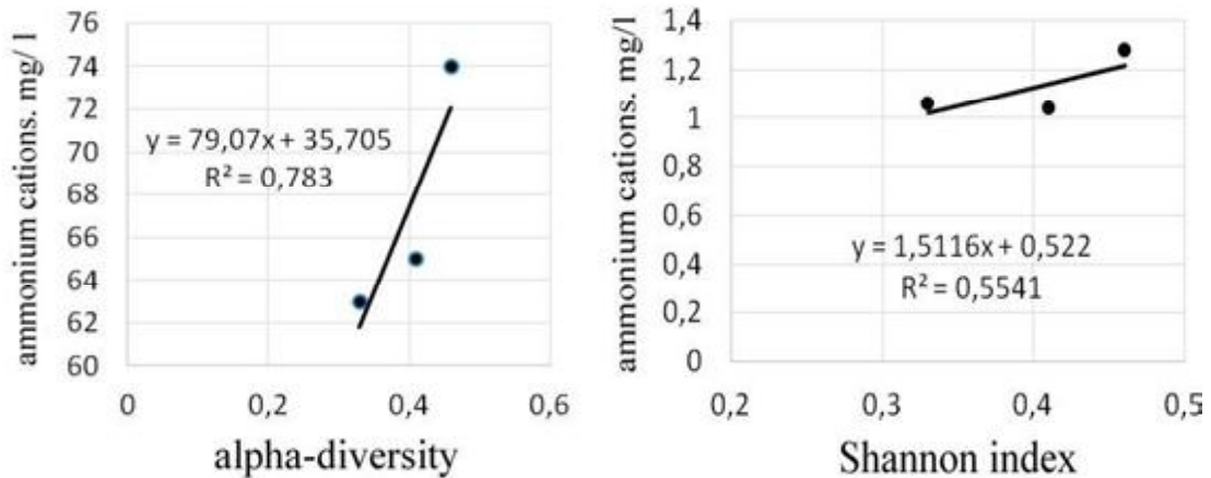
Figure 1. Dependence of biological indicators of macrophyte communities on the concentration of ammonium ions ( \text{NH}_4^+ )
