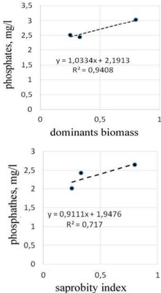
Figure 3. Dependence of biological indicators of macrophyte communities on phosphate ions ( \text{PO}_4^{3-} ) concentration
