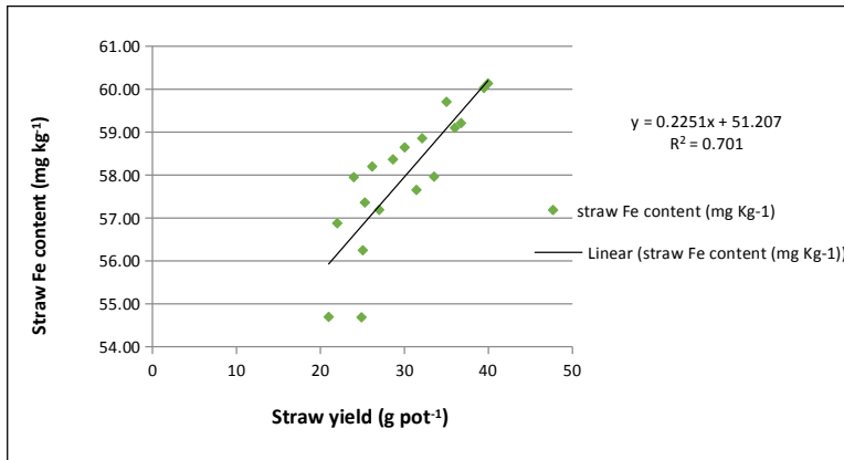
Fig.2. Linear relationship between straw yield and straw Fe content
